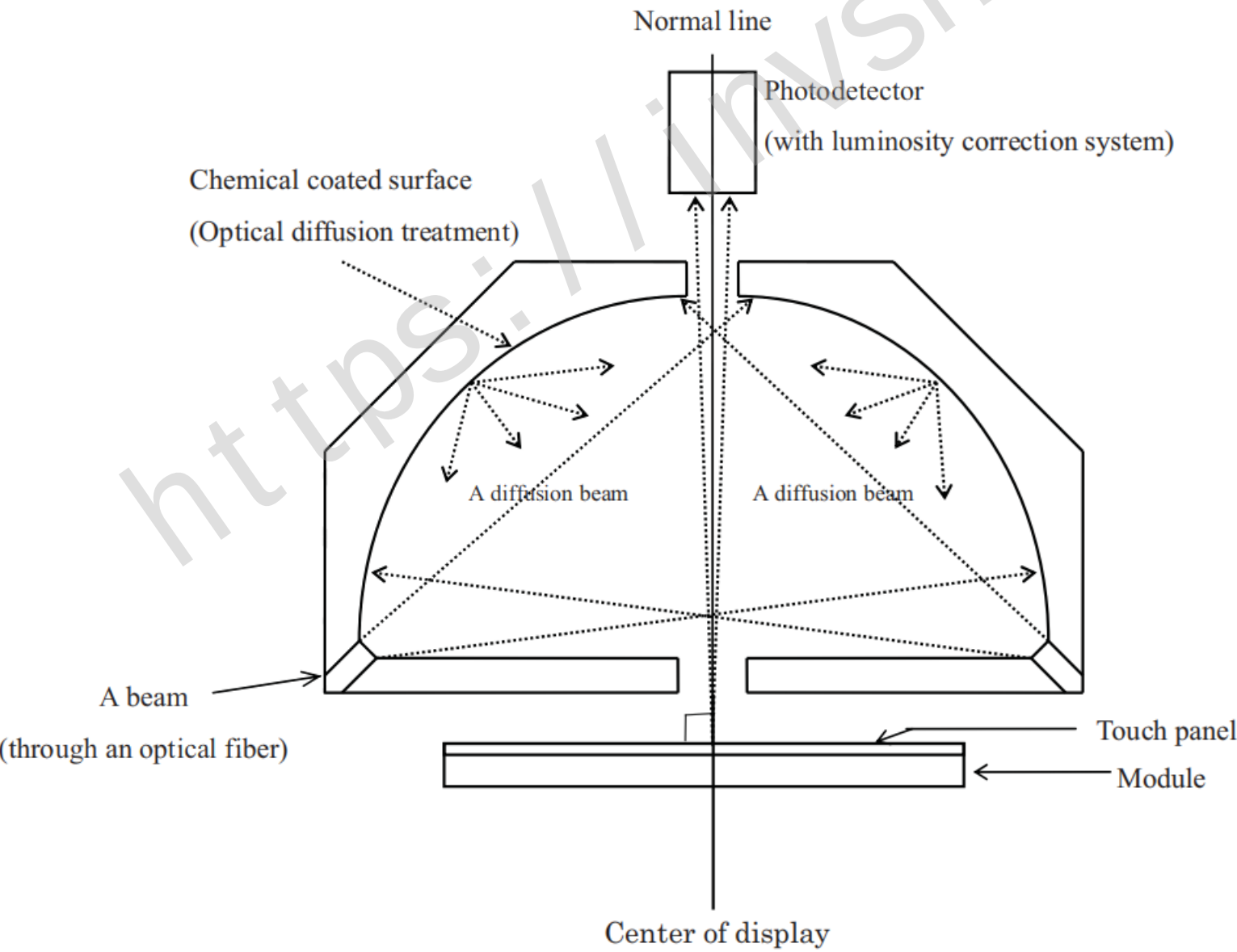
Measuring method (a) for optical characteristics
