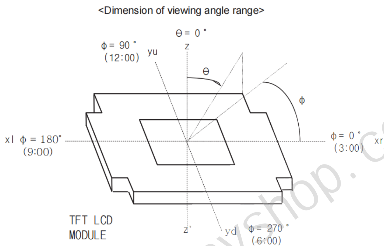
FIG. 4 Viewing angle
