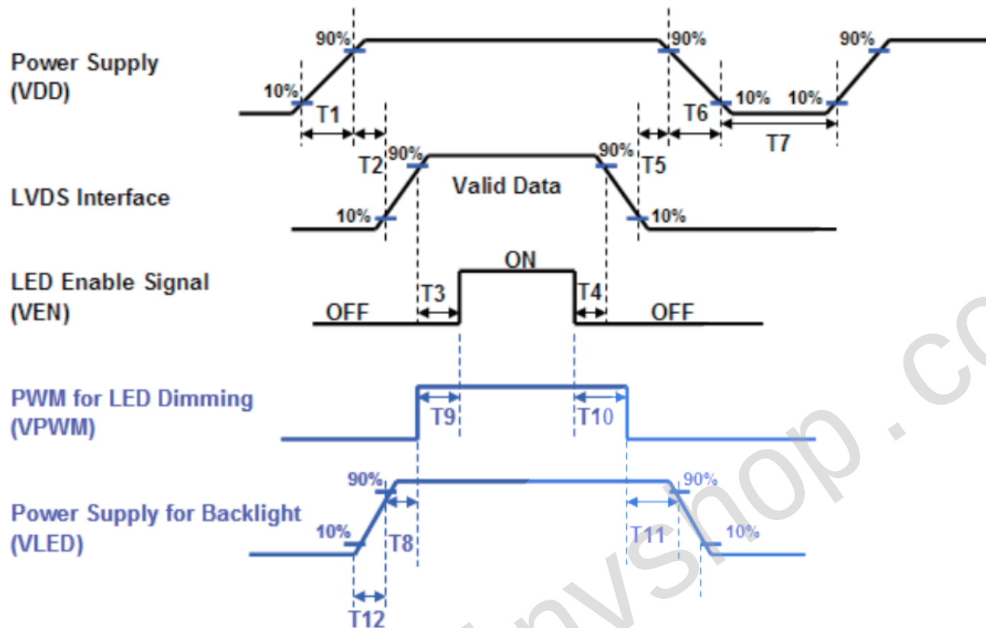
Power ON/OFF sequence timing
