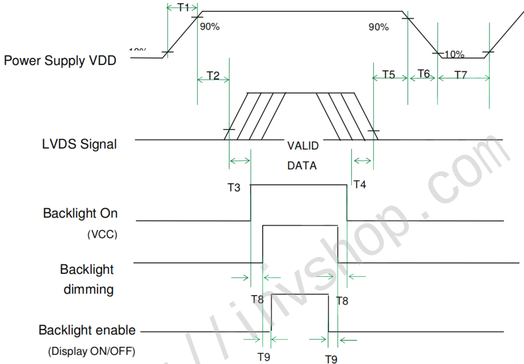
Power ON/OFF sequence timing
