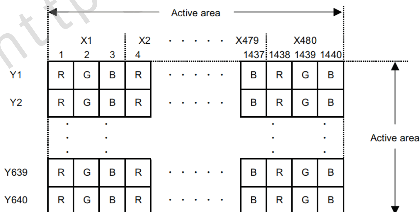
Dot arrangement (FPC cable placed leftside)
