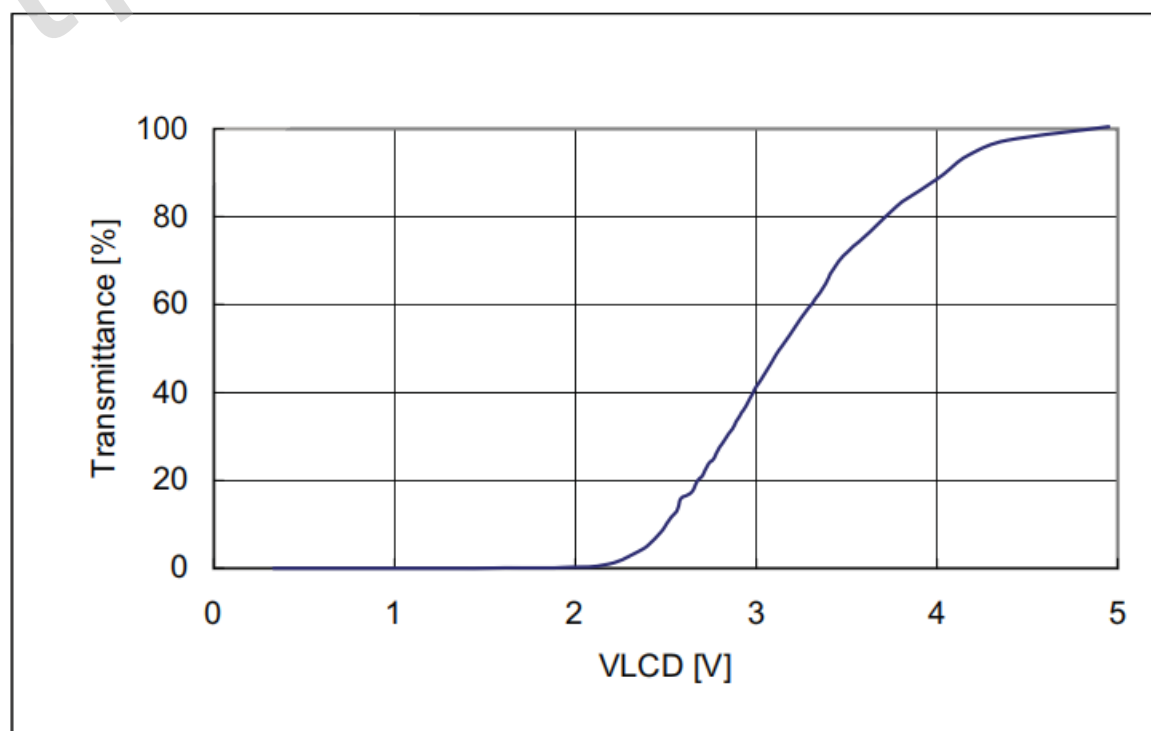
White V-T Curve
