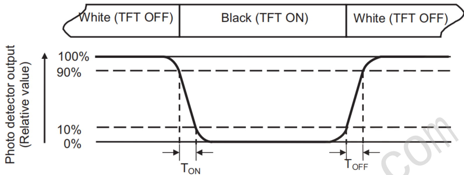
Fig. 4-3 Definition of response time
