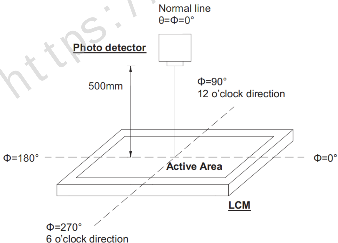
Fig. 4-2 Optical measurement system setup
