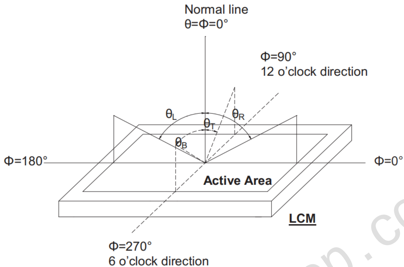
Fig. 4-1 Definition of viewing angle
