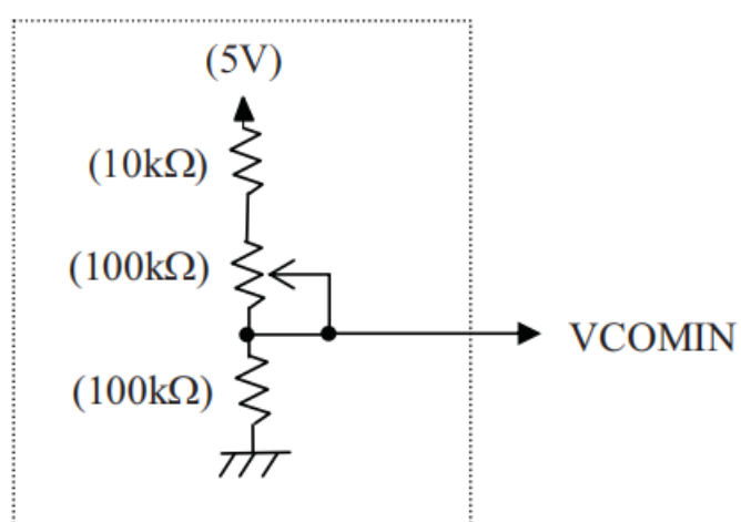
Reference design of COM circuit
