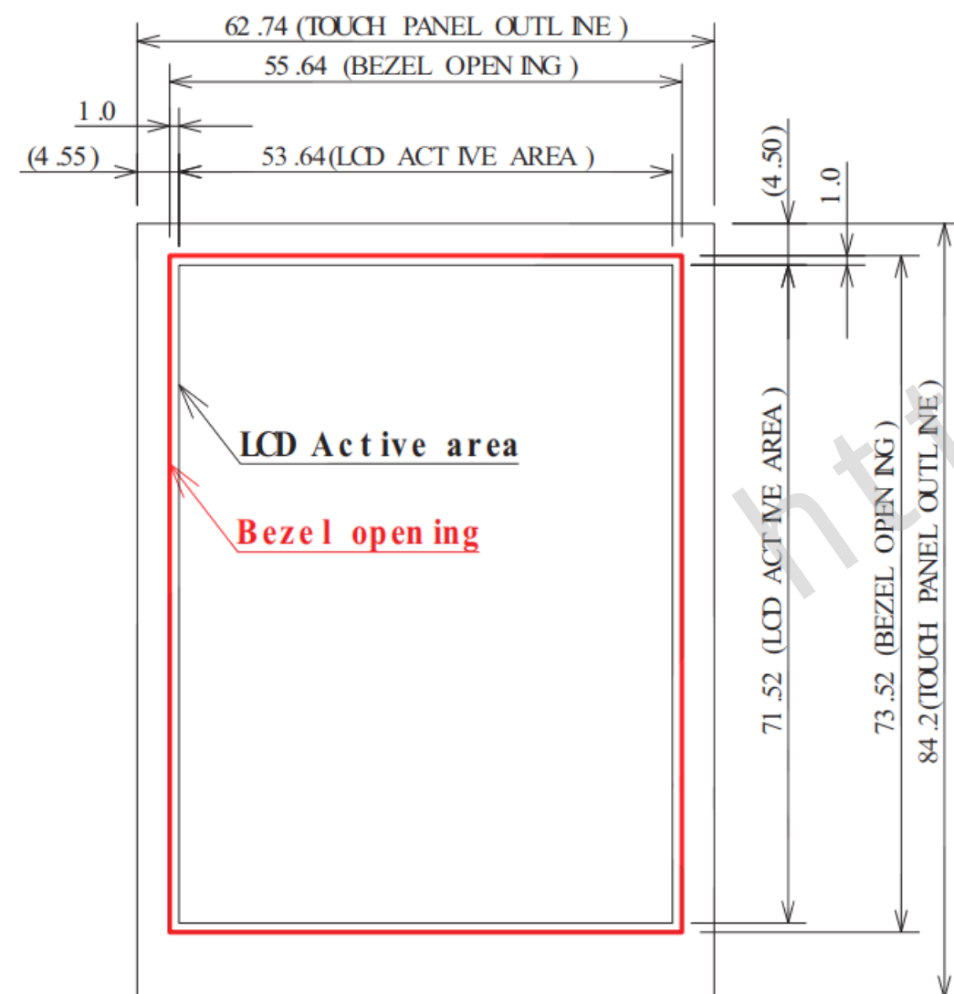
Front Bezel opening design
