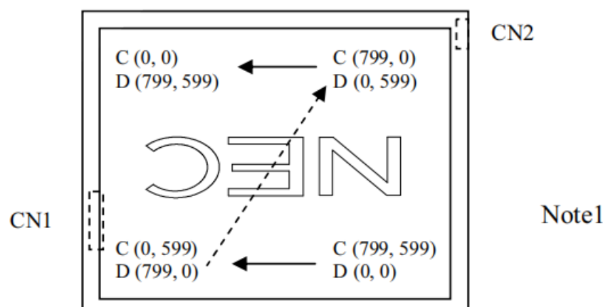
Figure2. Reverse scan (DPS: High)
