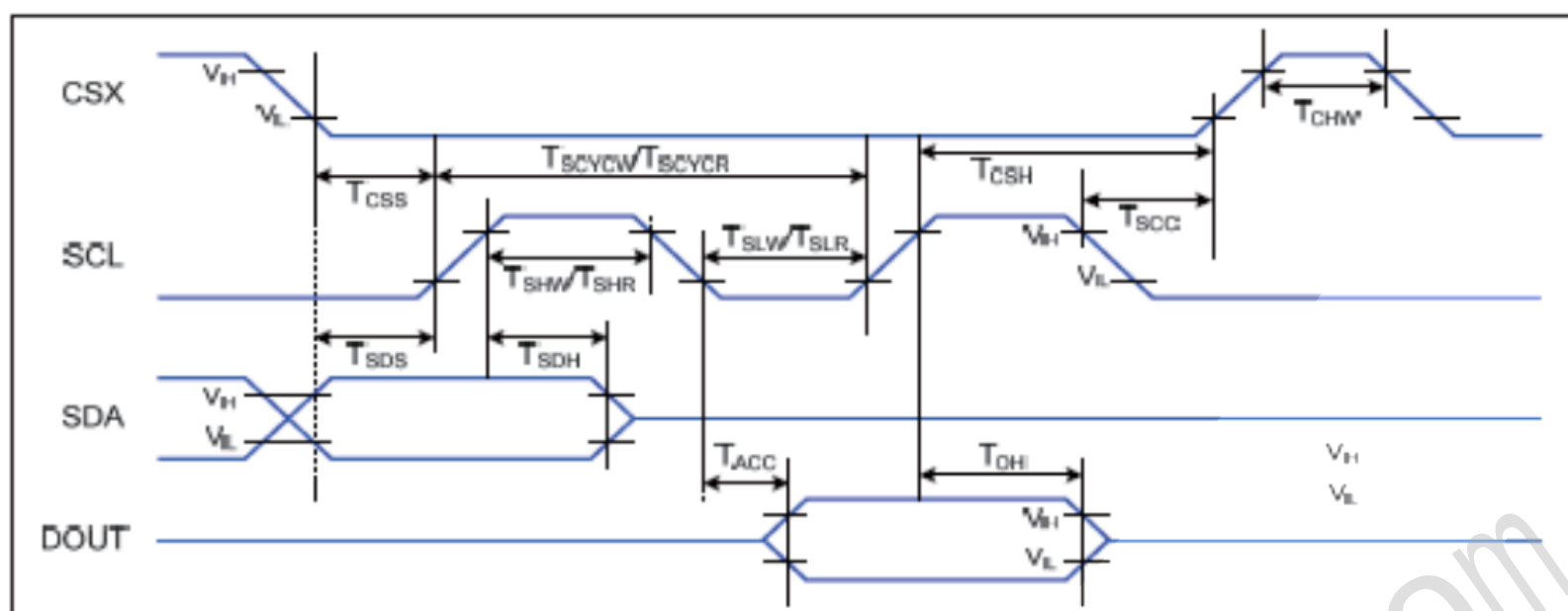
Figure 4 3-line serial Interface Timing Characteristics
