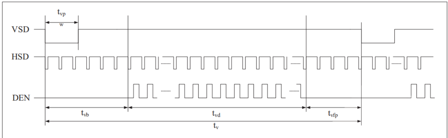
Figure 5.2.3 Vertical Input Timing Diagram
