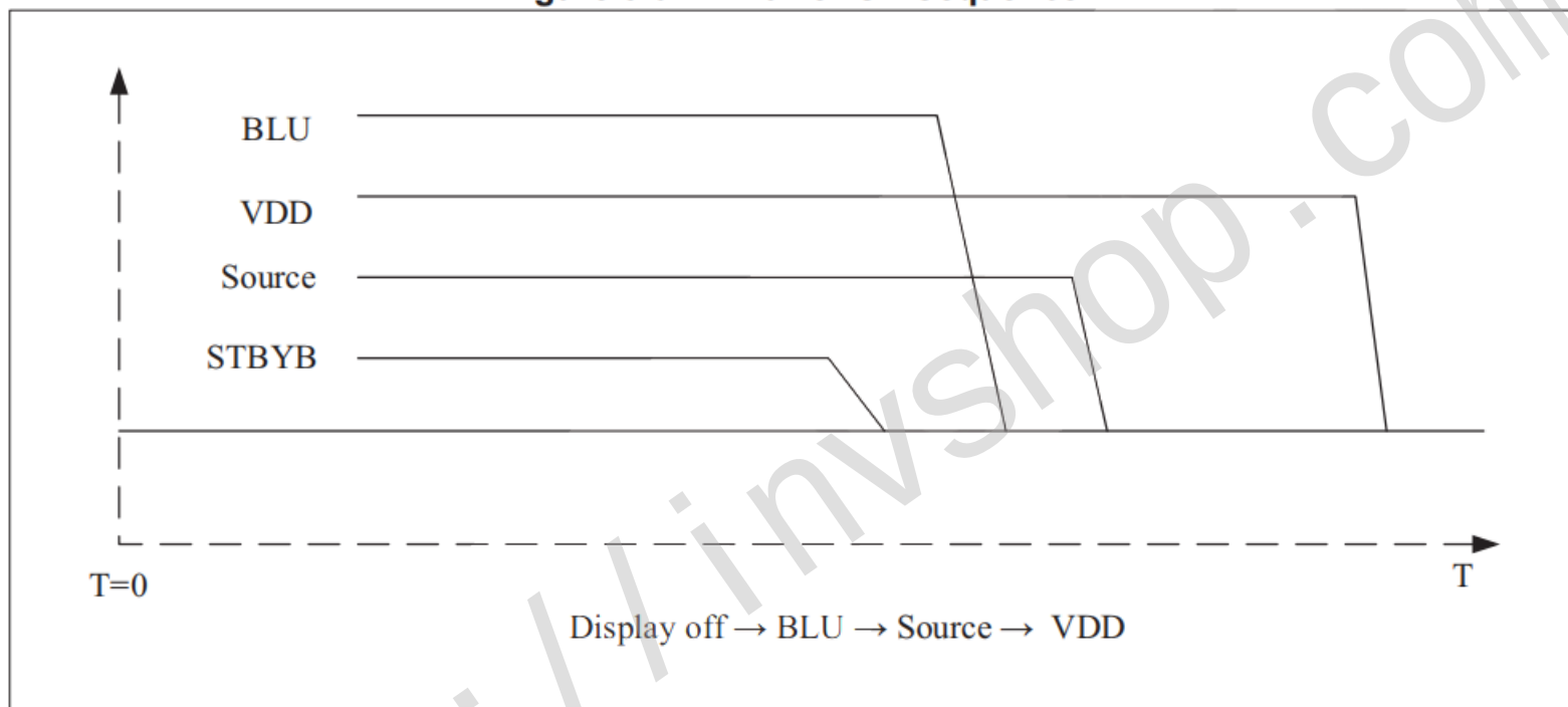
Figure 5.3.3 Power Off Sequence
