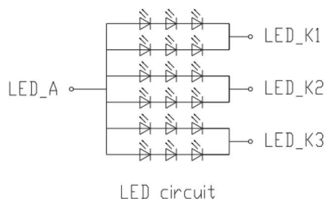
Figure 4.2 LED connection of backlight
