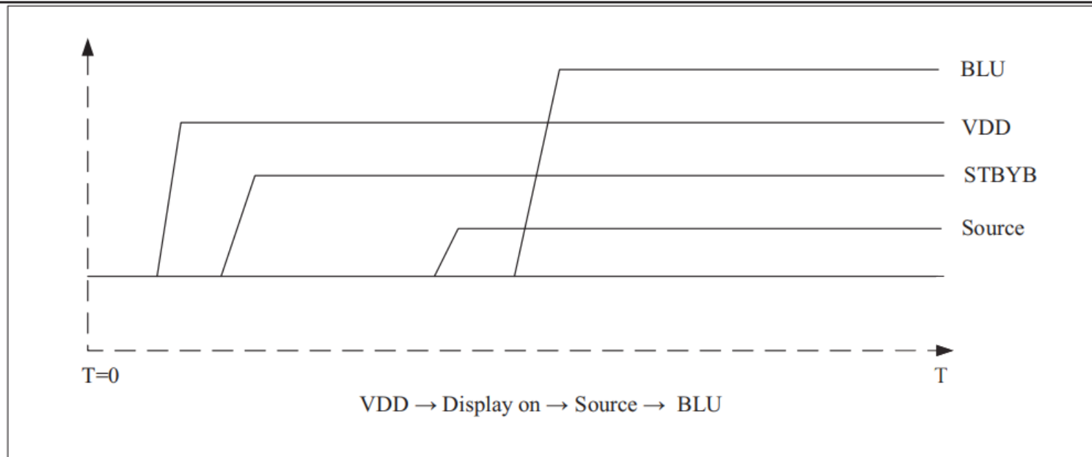
Figure 5.3.2 Power On Sequence
