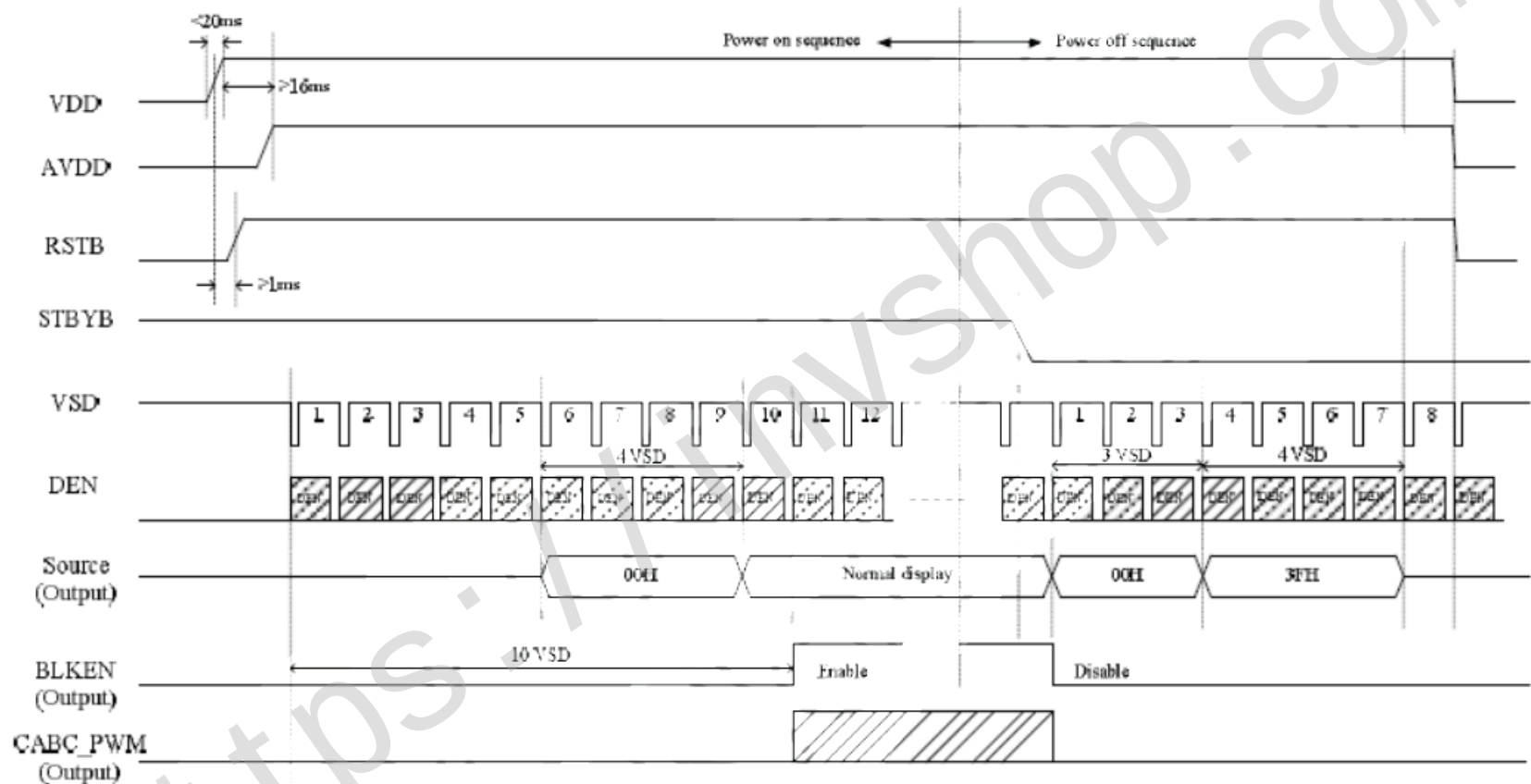
Figure 5.3.1 Power On/Off Sequence
