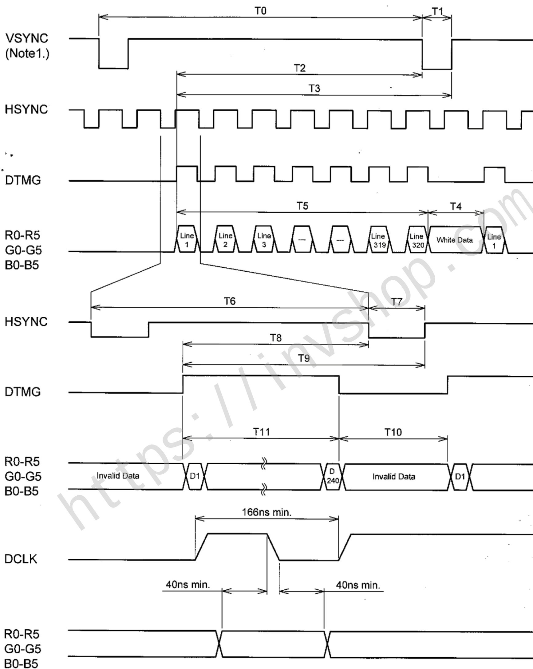
Fig1. Timing sequence for Graphic controller
