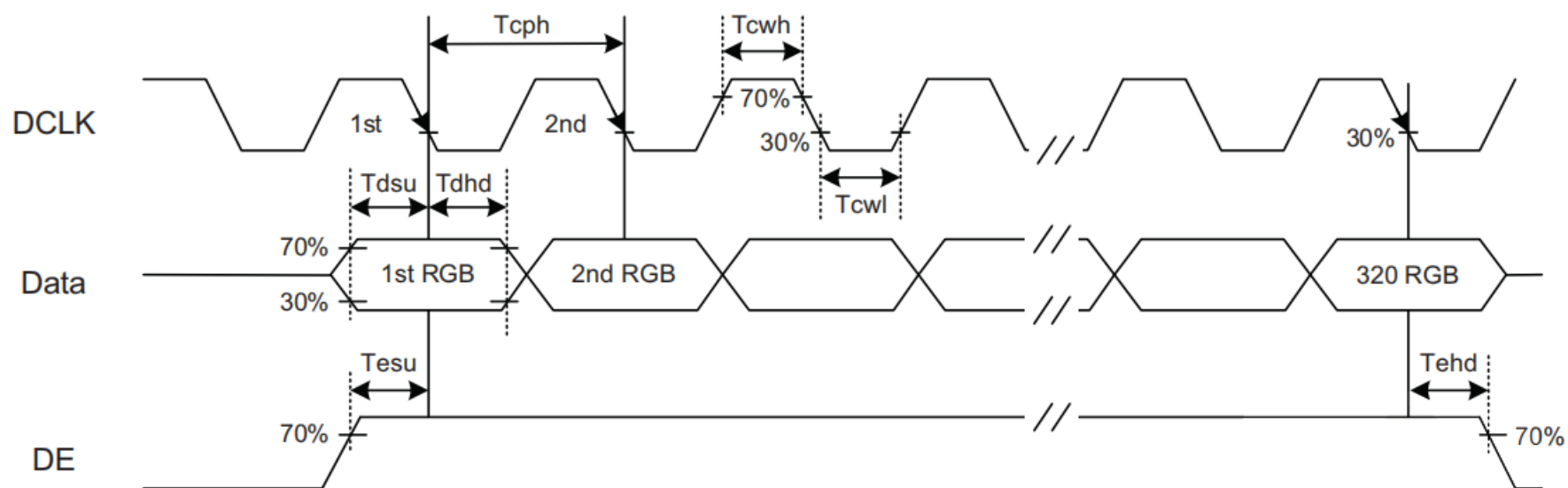
Fig. 9.3 Setup & Hold Time
