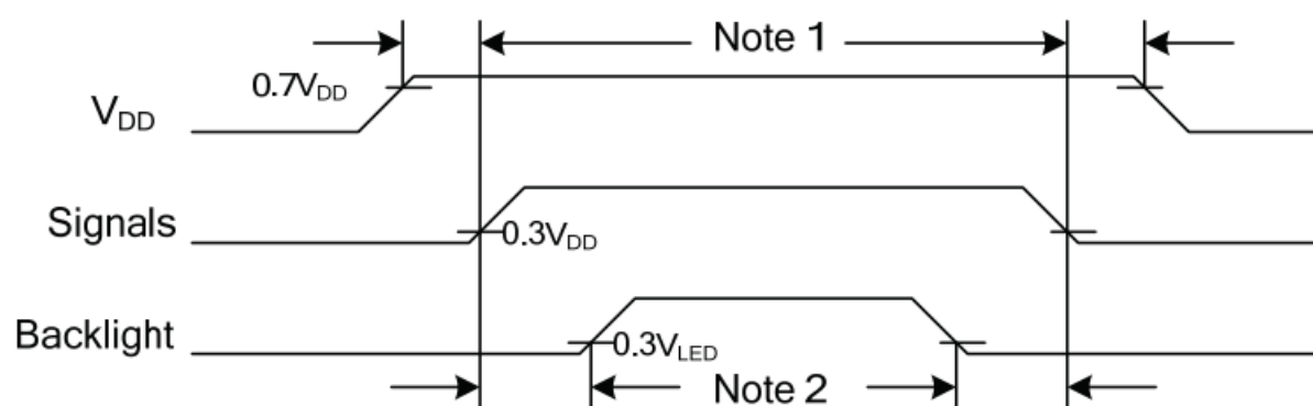
Fig. 9.4 Power Sequence Timing
