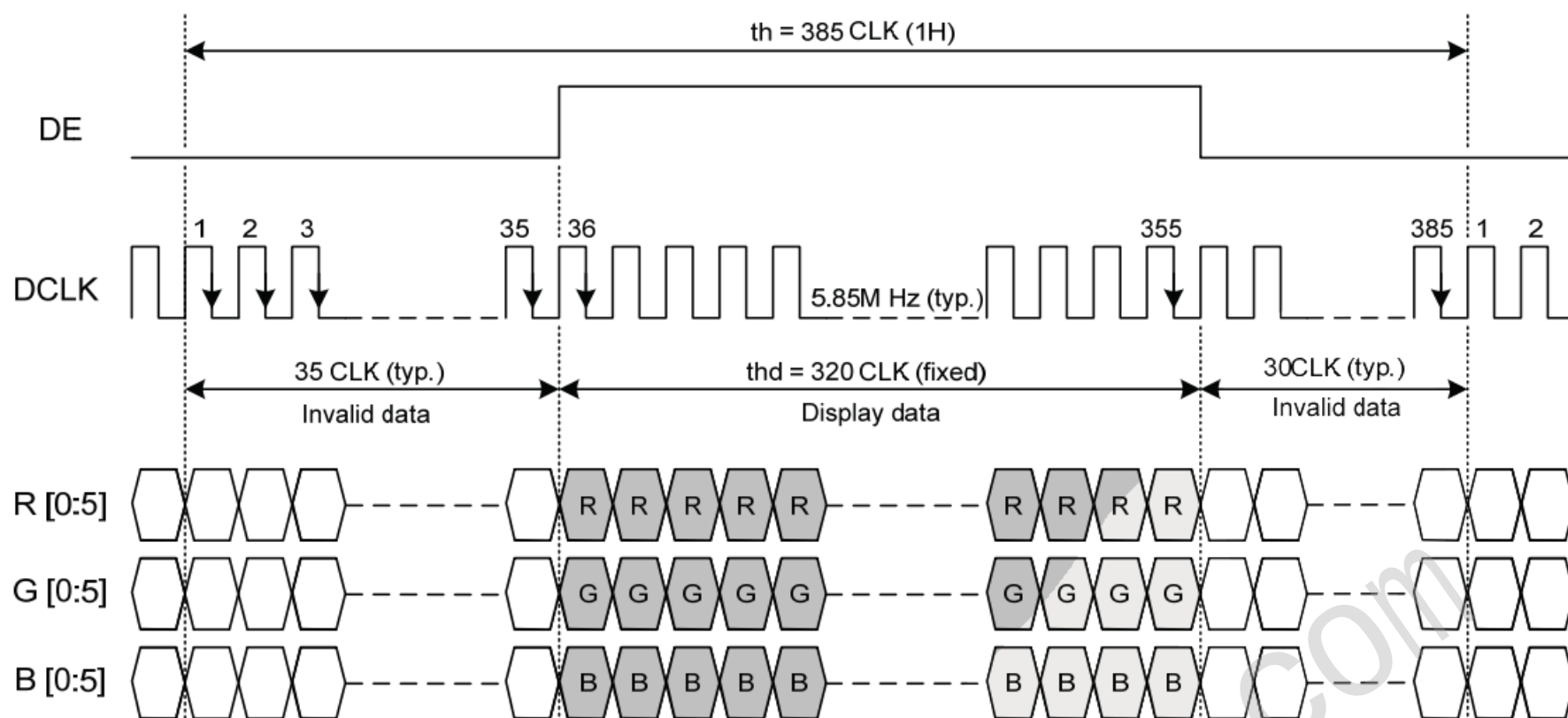
Fig. 9.1 Horizontal Timing
