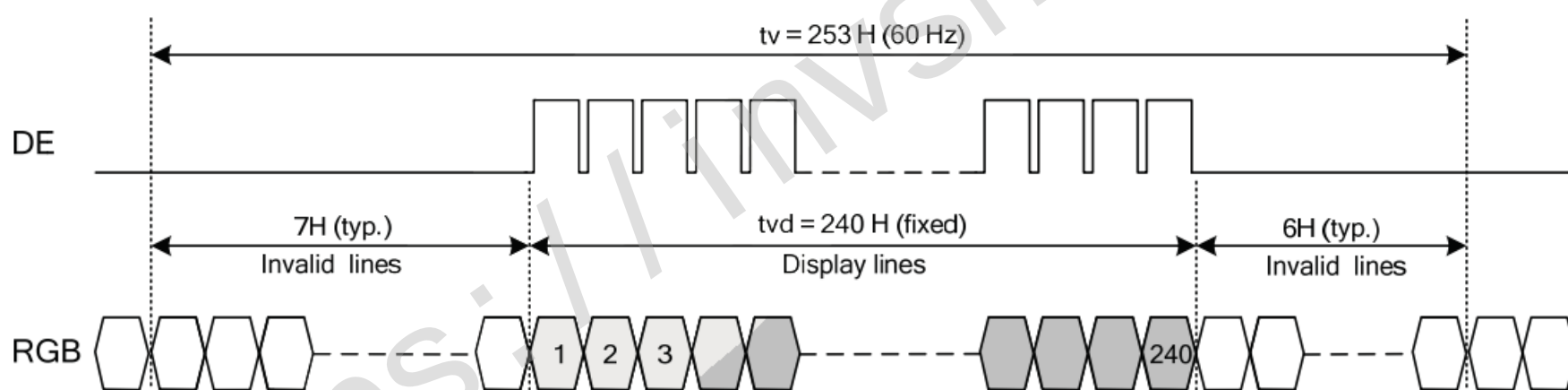
Fig. 9.2 Vertical Timing
