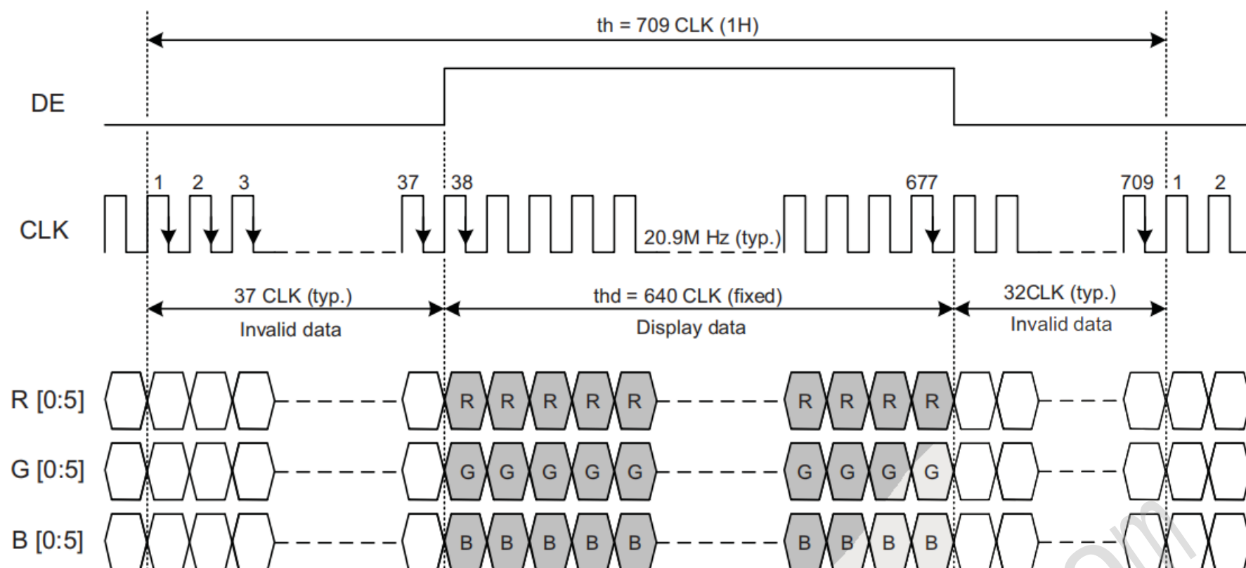
Fig. 9.3 Horizontal Timing
