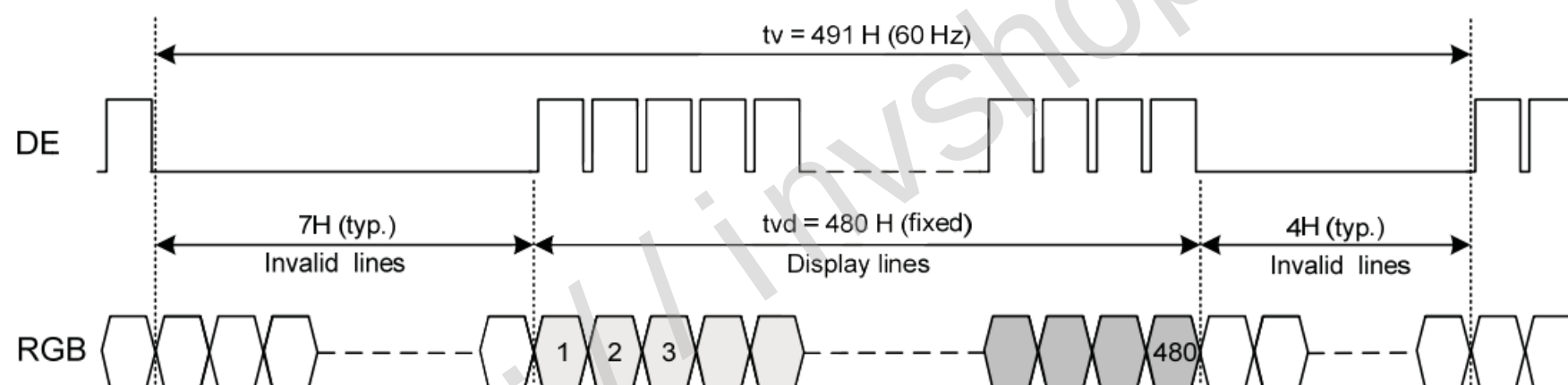
Fig. 9.4 Vertical Timing
