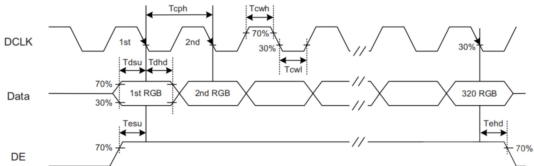
Fig. 9.5 Setup & Hold Time
