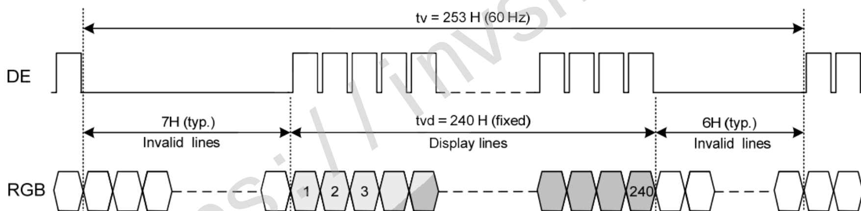
Fig. 9.2 Vertical Timing
