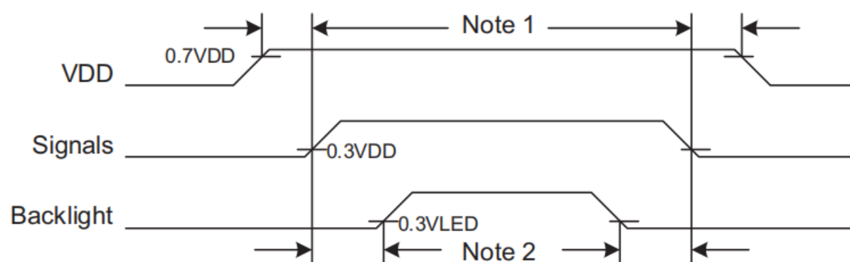
Fig. 8.7 Power Sequence Timing
